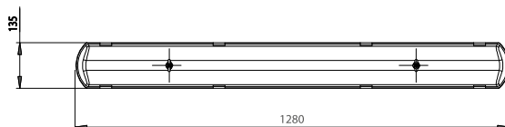
рис. 2 LAD LED LINE-OZ-40/60/80
