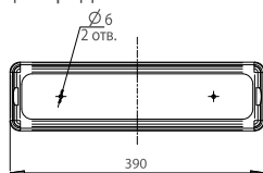
рис. 1 LAD LED LINE-OZ-15/25
